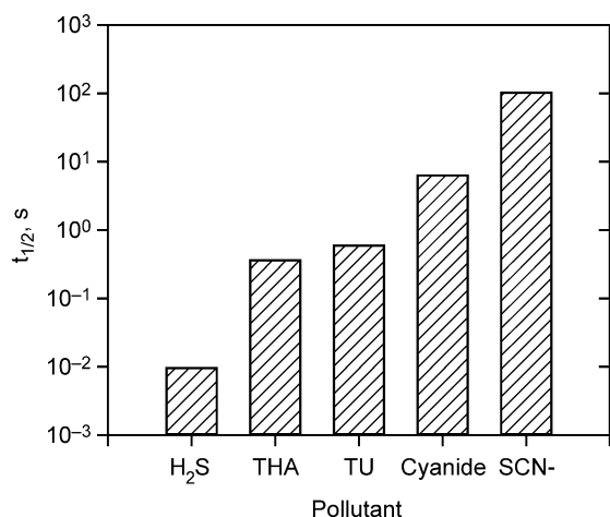
Figure 1 | Half-lives of the reactions between Fe(VI) (500 \mu M) and pollutants (100 \mu M) at pH 9 and 25 °C (THA, thioacetamide; TU, thiourea).
